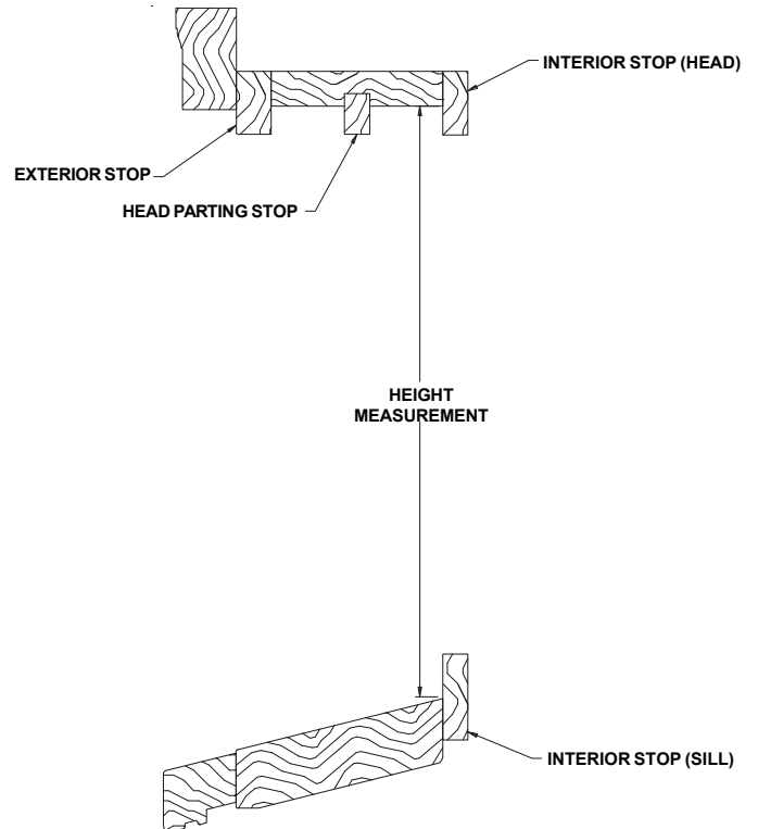
EXISTING WINDOW FRAME –Fig. 2
